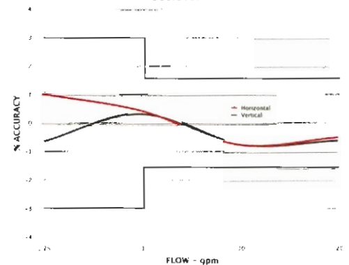
ACCURACY CURVE
